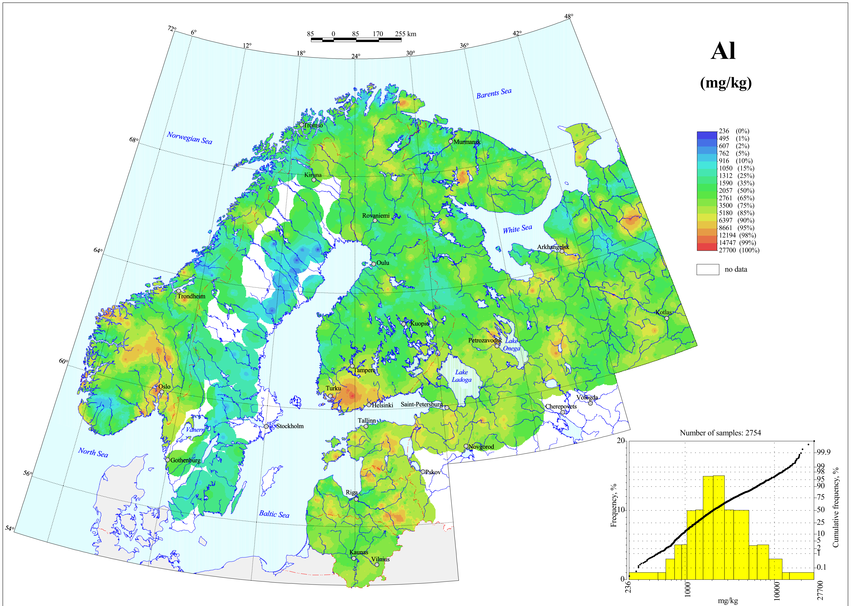
Aluminium in Organic Soil Layer, Total Content
